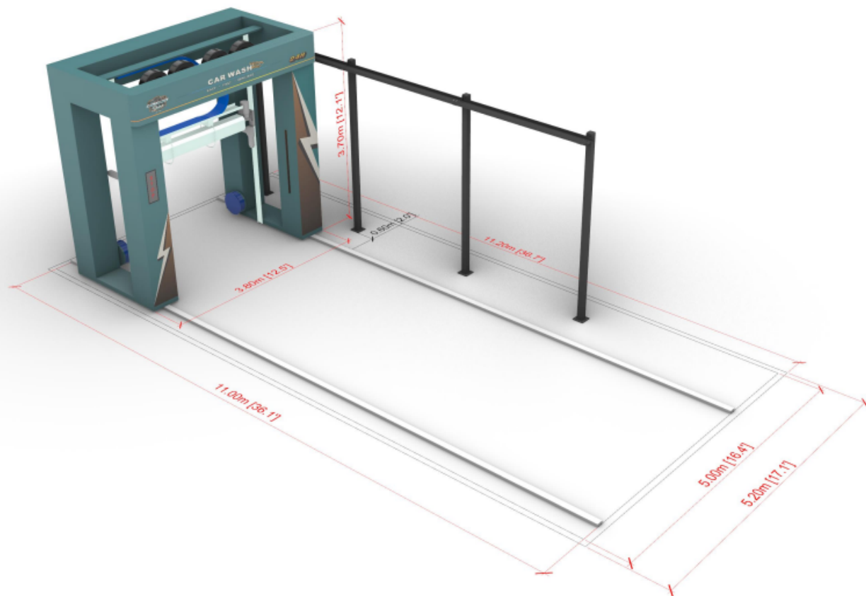
Touchless Car Wash Machine LT V2.0 3D Diagramm - 2
